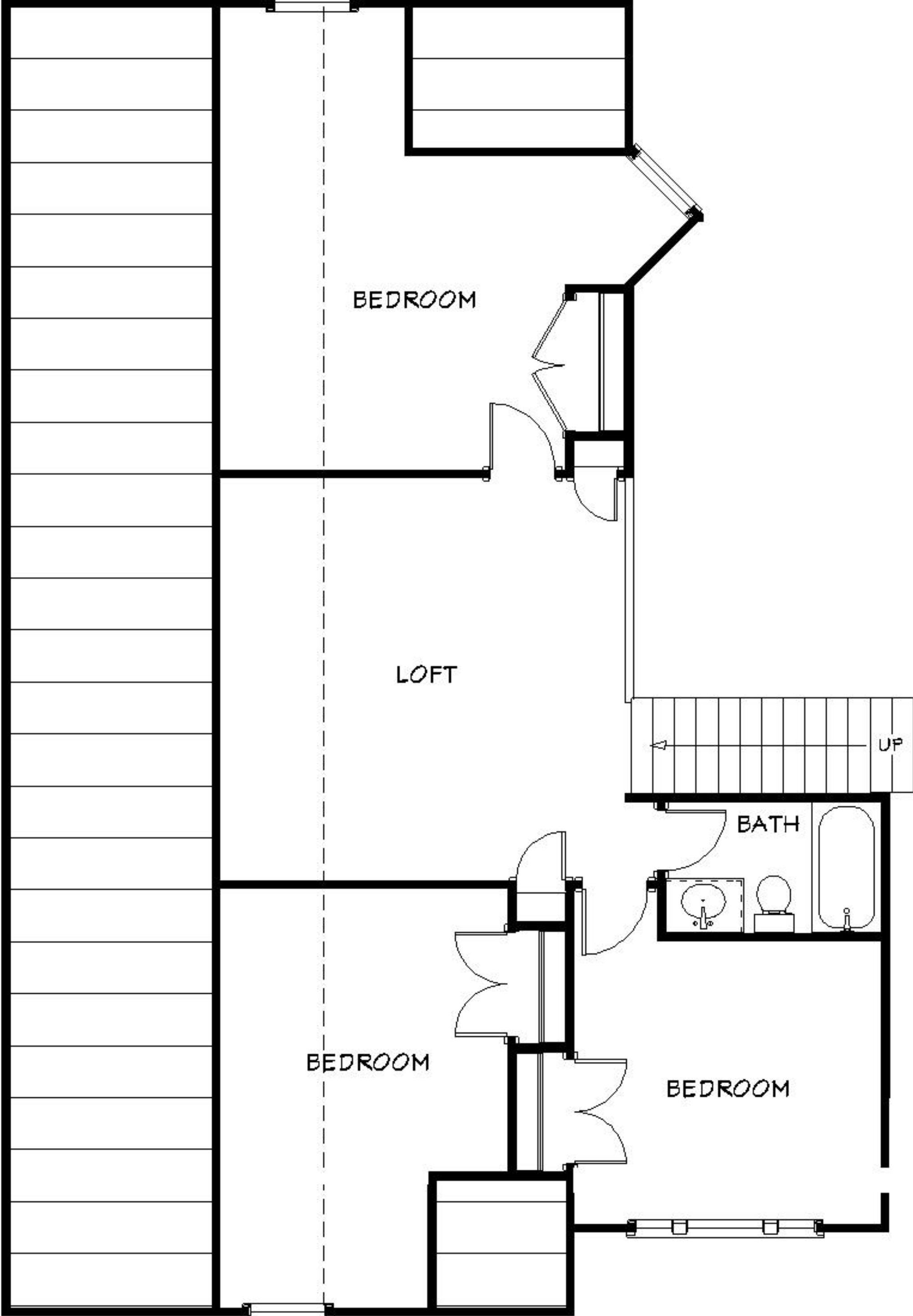
UPPER FLOOR 916 Square Feet
