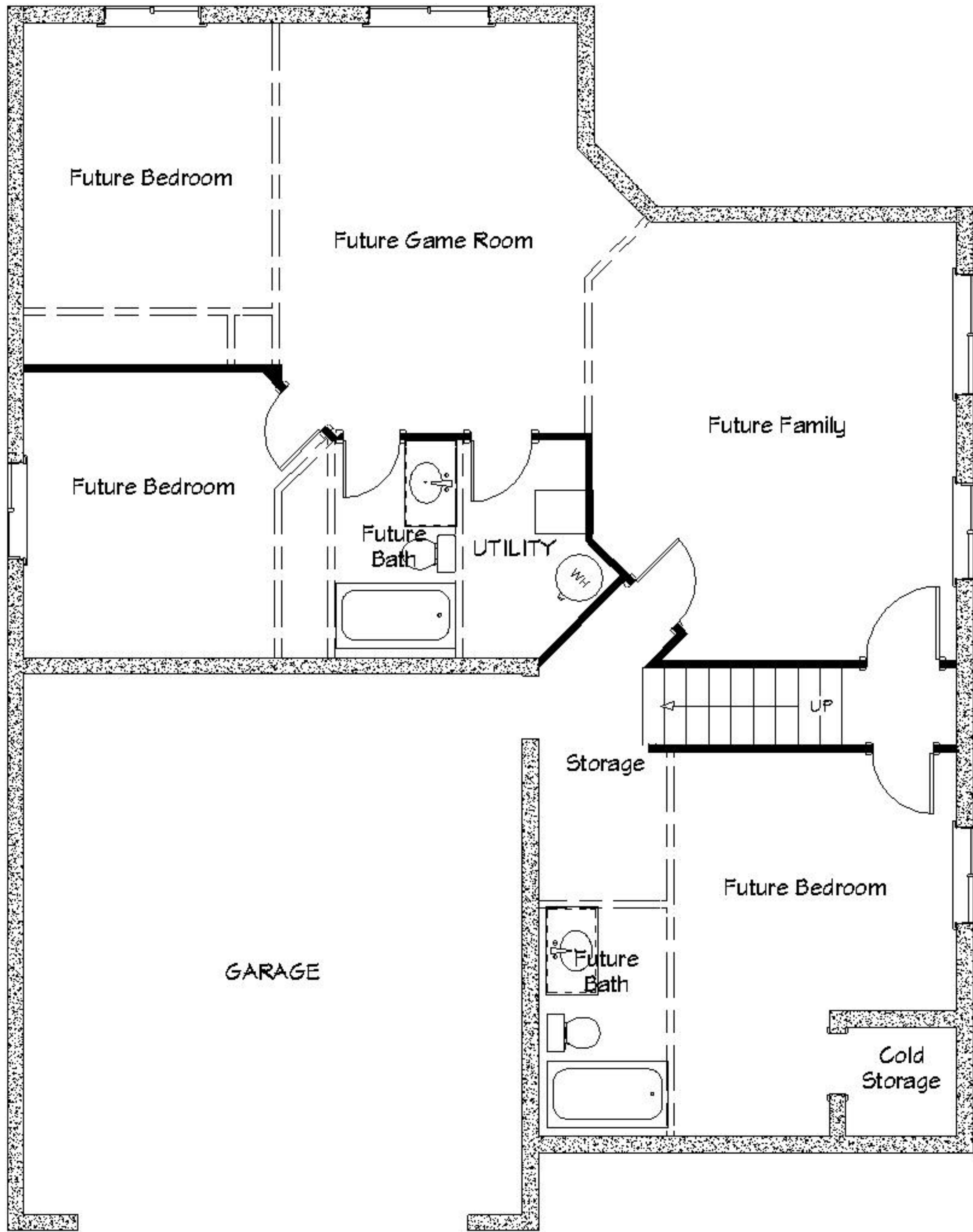
BASEMENT 1350 Square Feet
