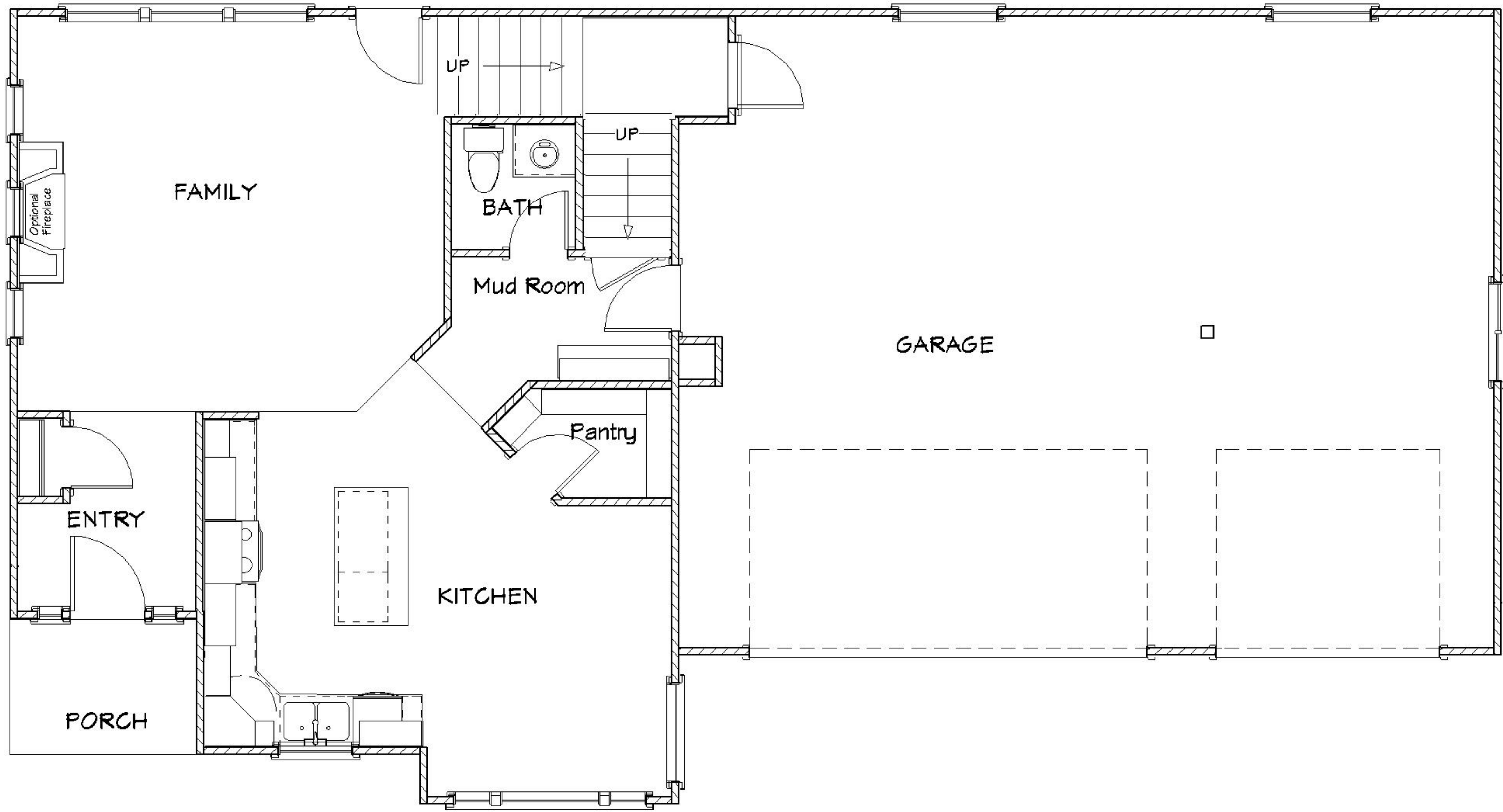
MAIN FLOOR 800 SQUARE FEET
