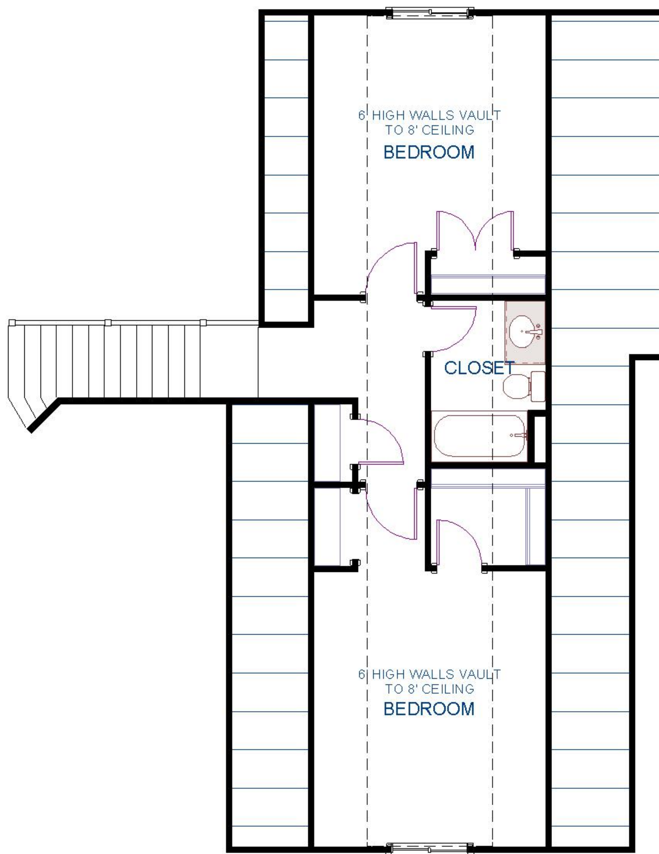
UPPER FLOOR PLAN 579 SQUARE FEET
