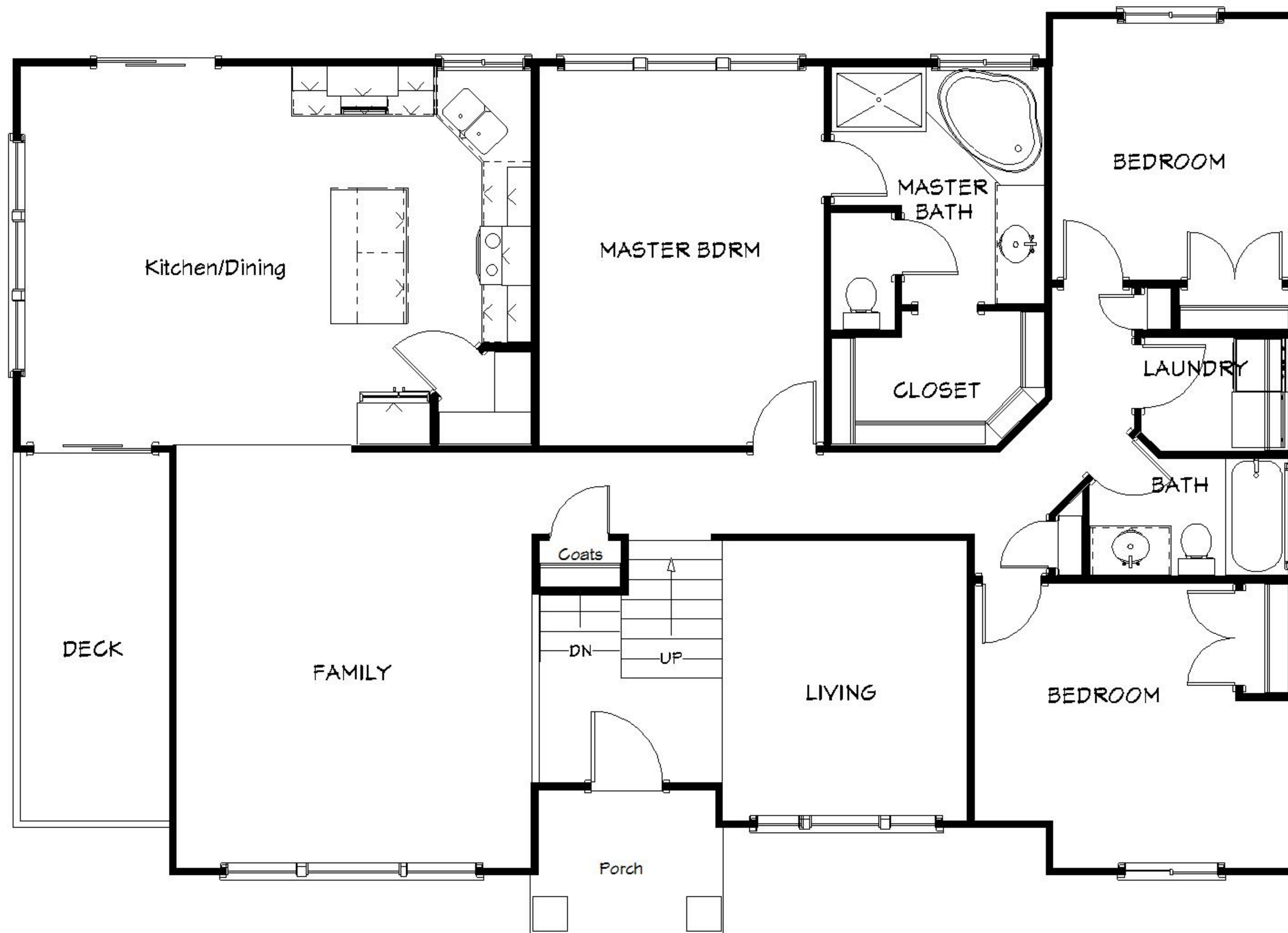
MAIN FLOOR PLAN 1730 Square Feet Width: 52'6" Depth: 34'7"
