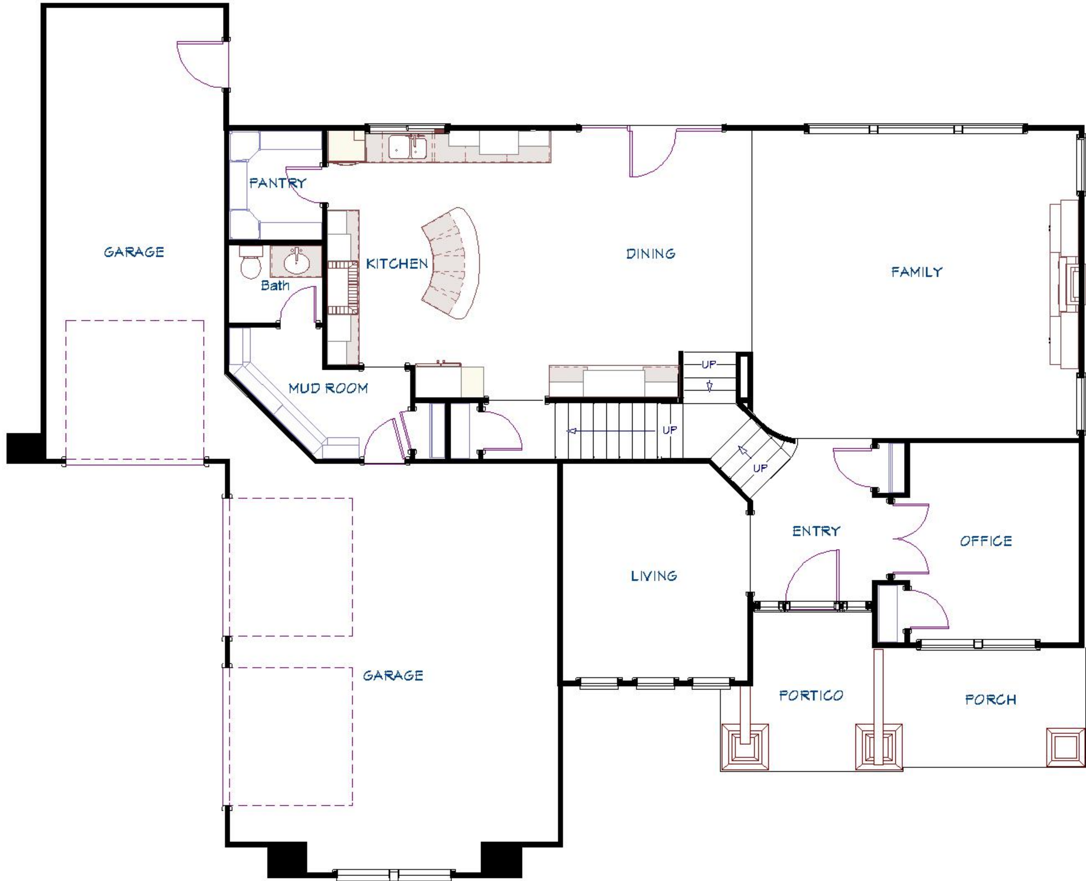
MAIN FLOOR 1645 SQUARE FEET WIDTH 68' DEPTH 55'
