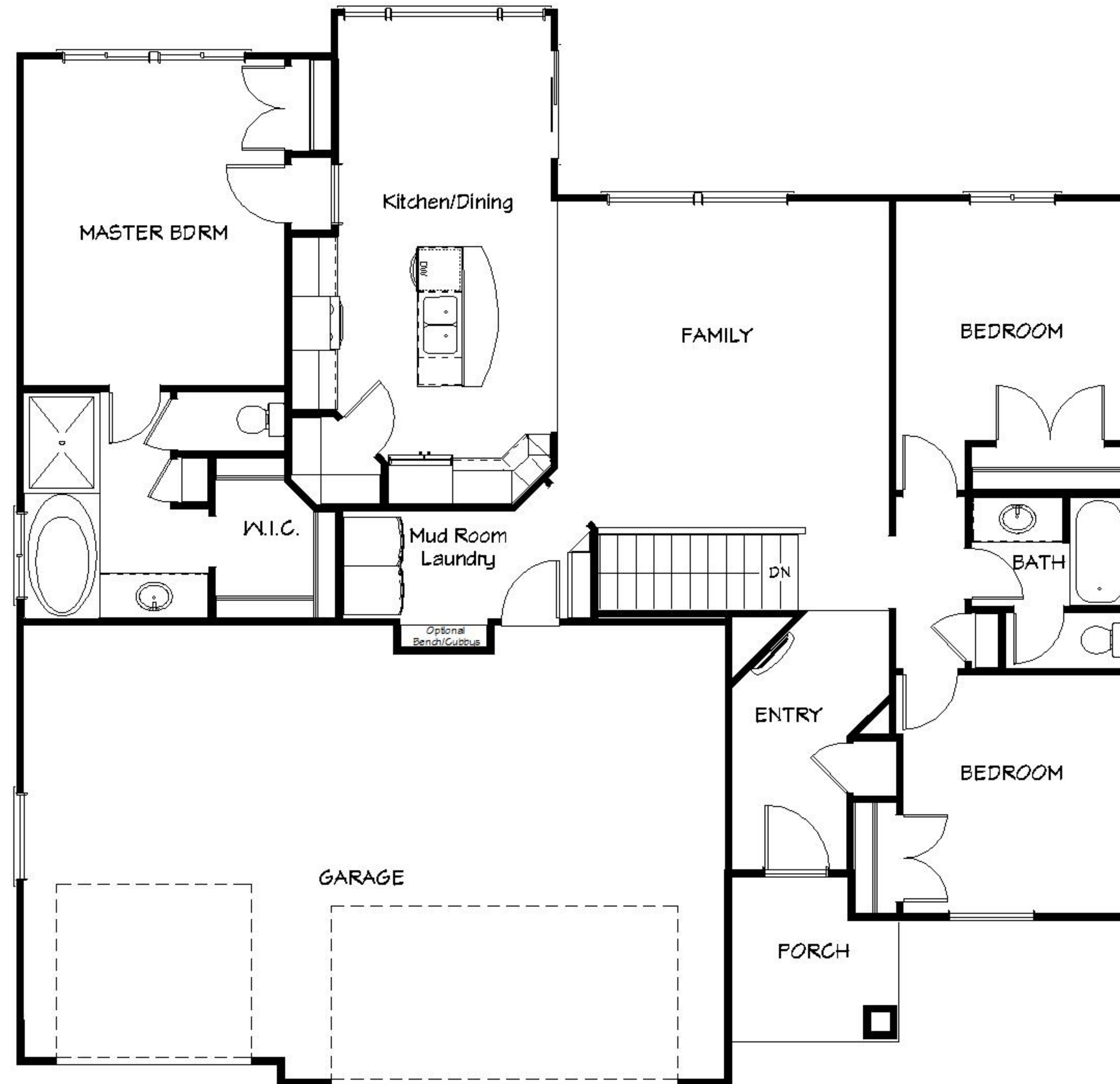
MAIN FLOOR PLAN 1474 Square Feet Width 51' 8" Depth 49' 9"
