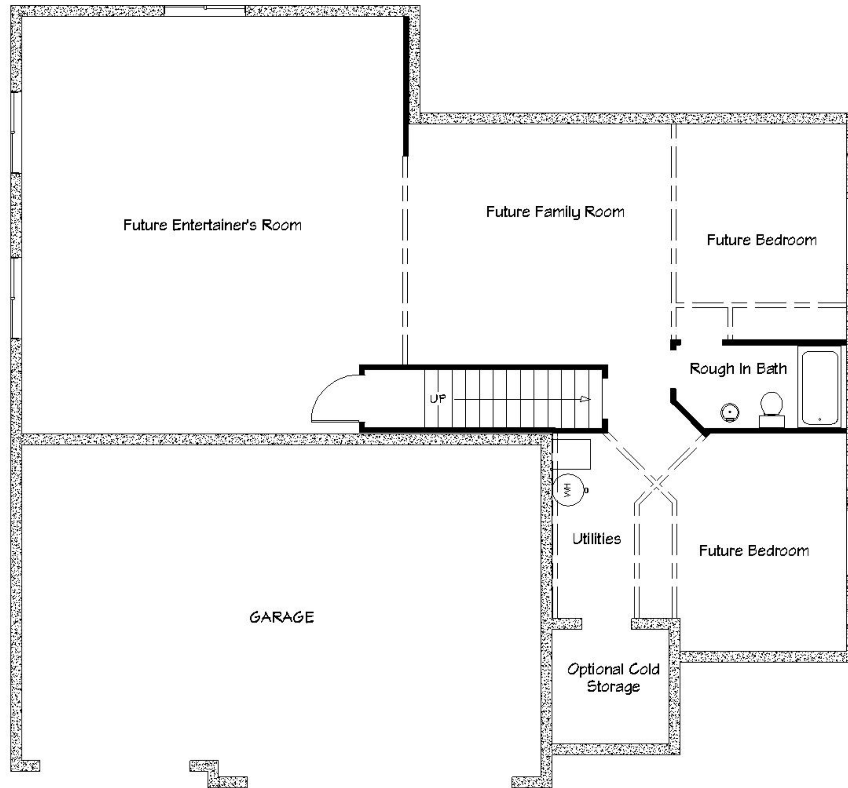
BASEMENT PLAN 1520 Square Feet
