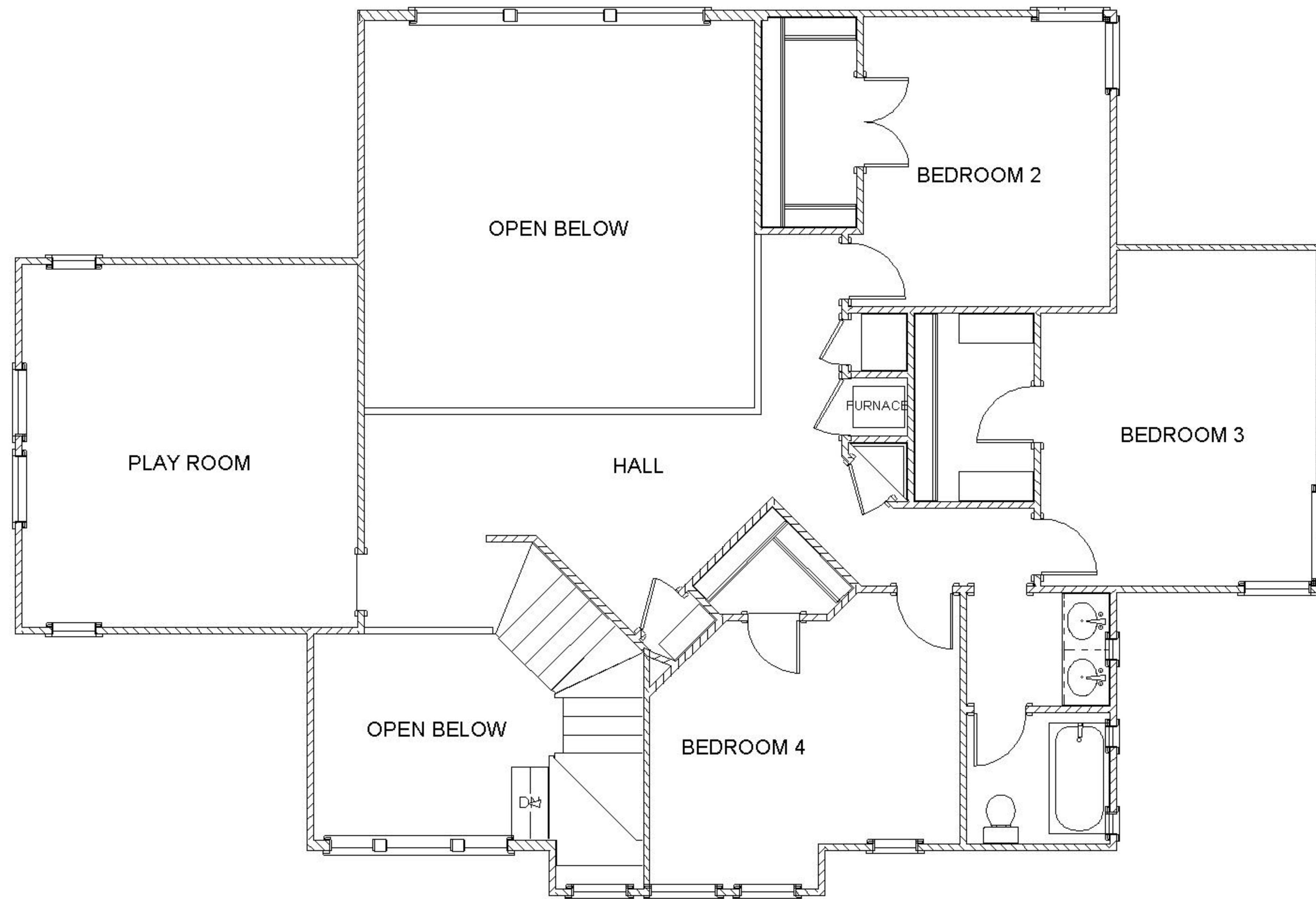
UPPER FLOOR PLAN 1326 SQUARE FEET
