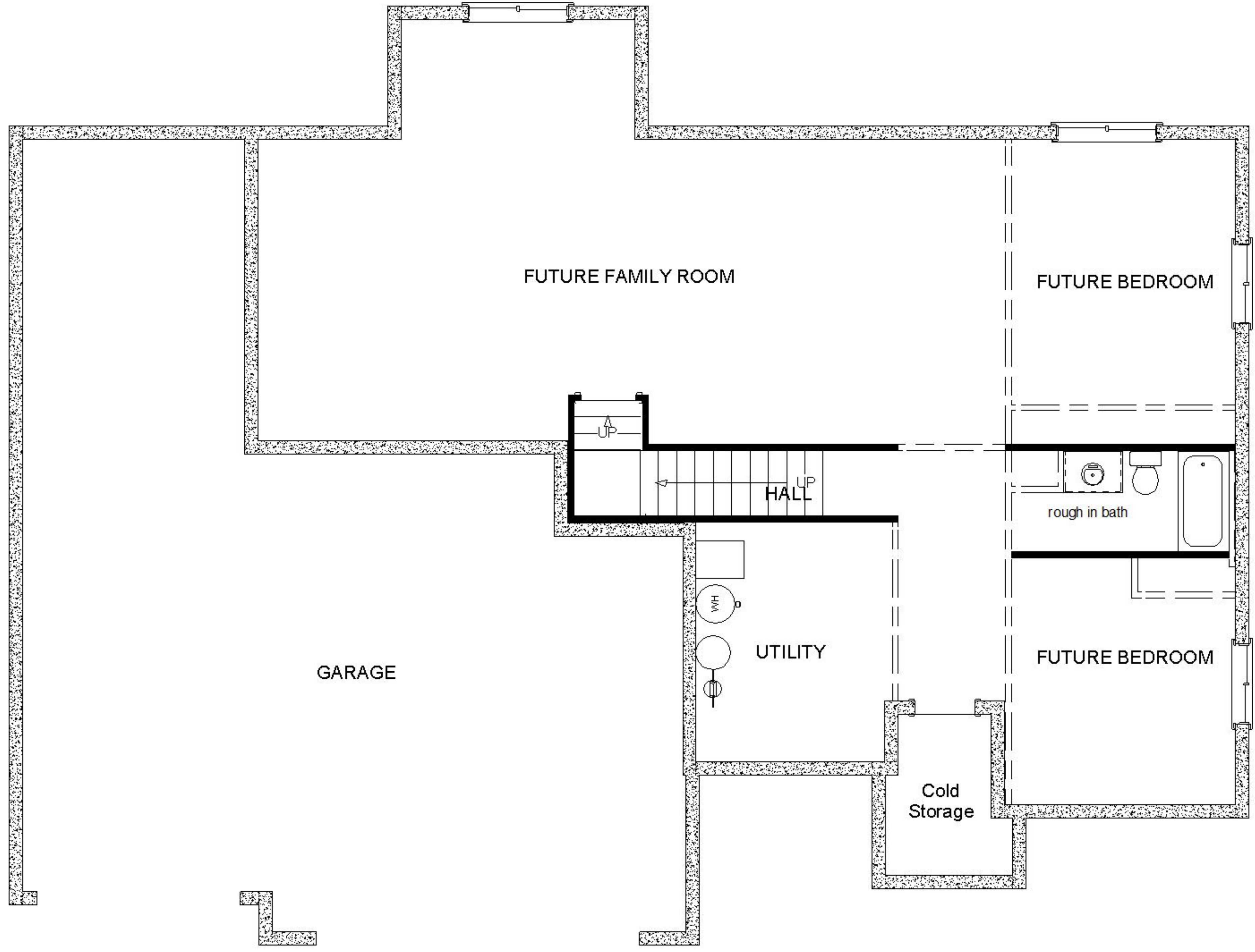
BASEMENT PLAN 1438 Square Feet
