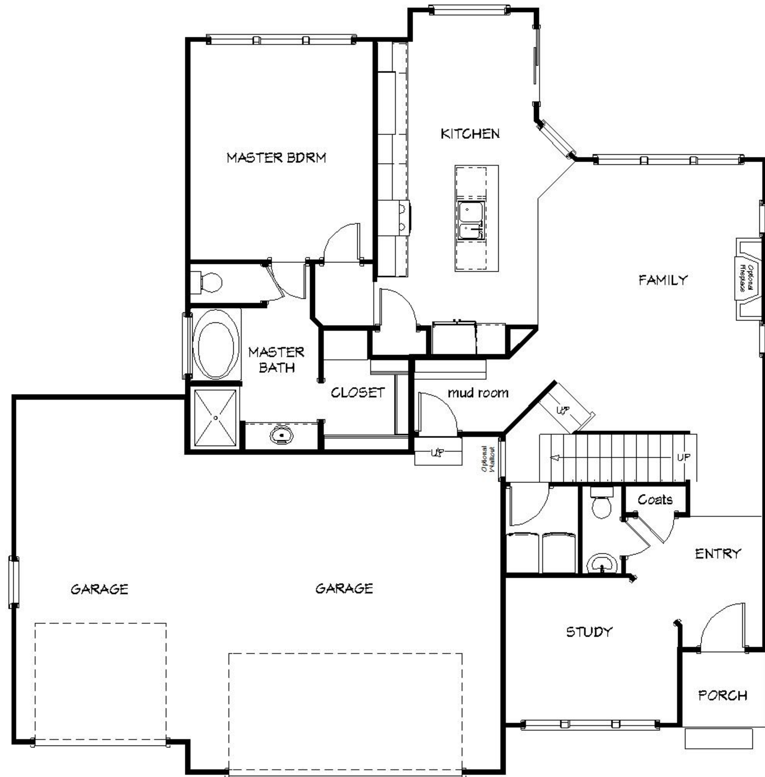
MAIN FLOOR PLAN 1344 Square Feet Width: 64' Depth: 52'9"
