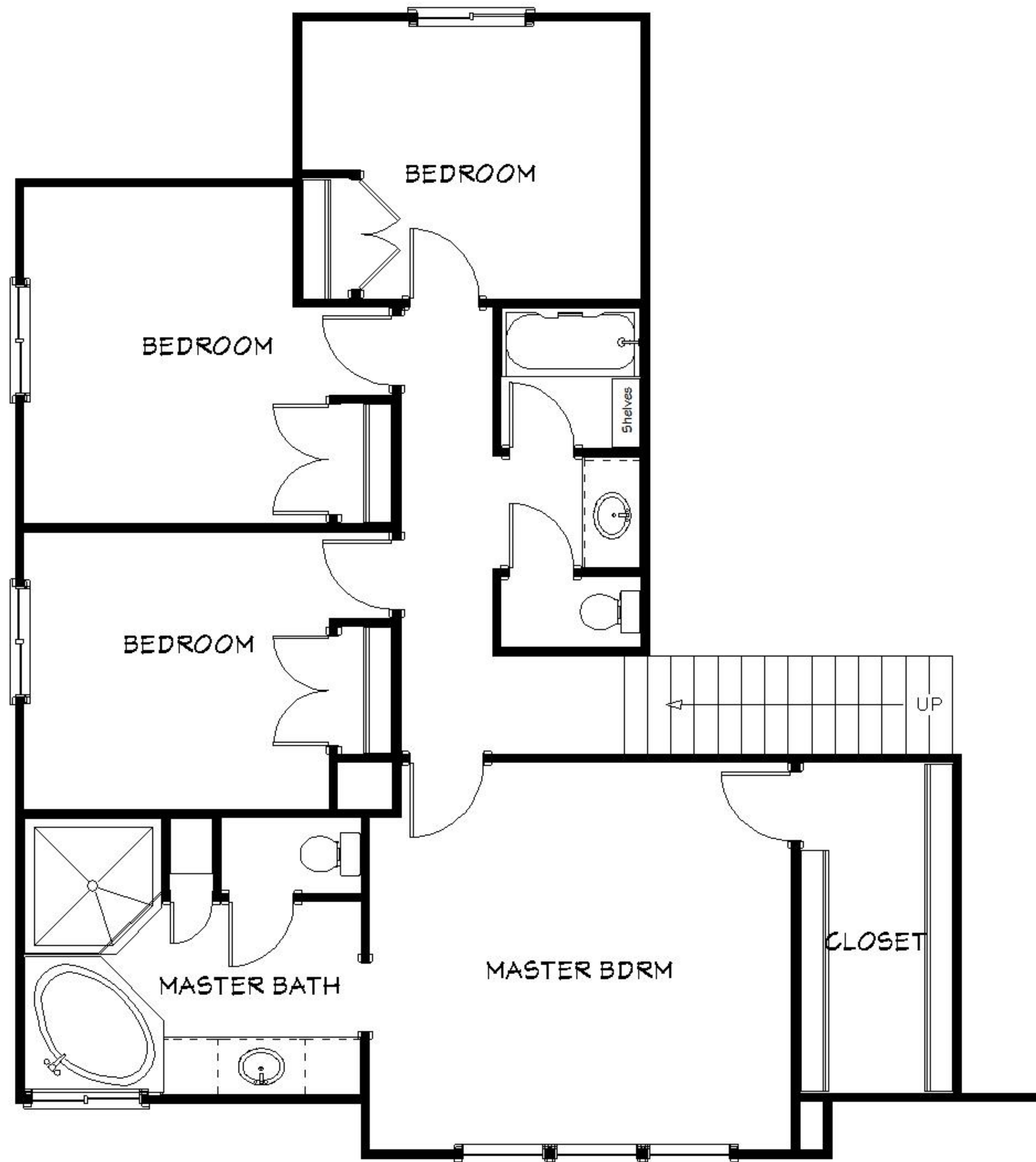
UPPER FLOOR PLAN 1040 Square Feet
