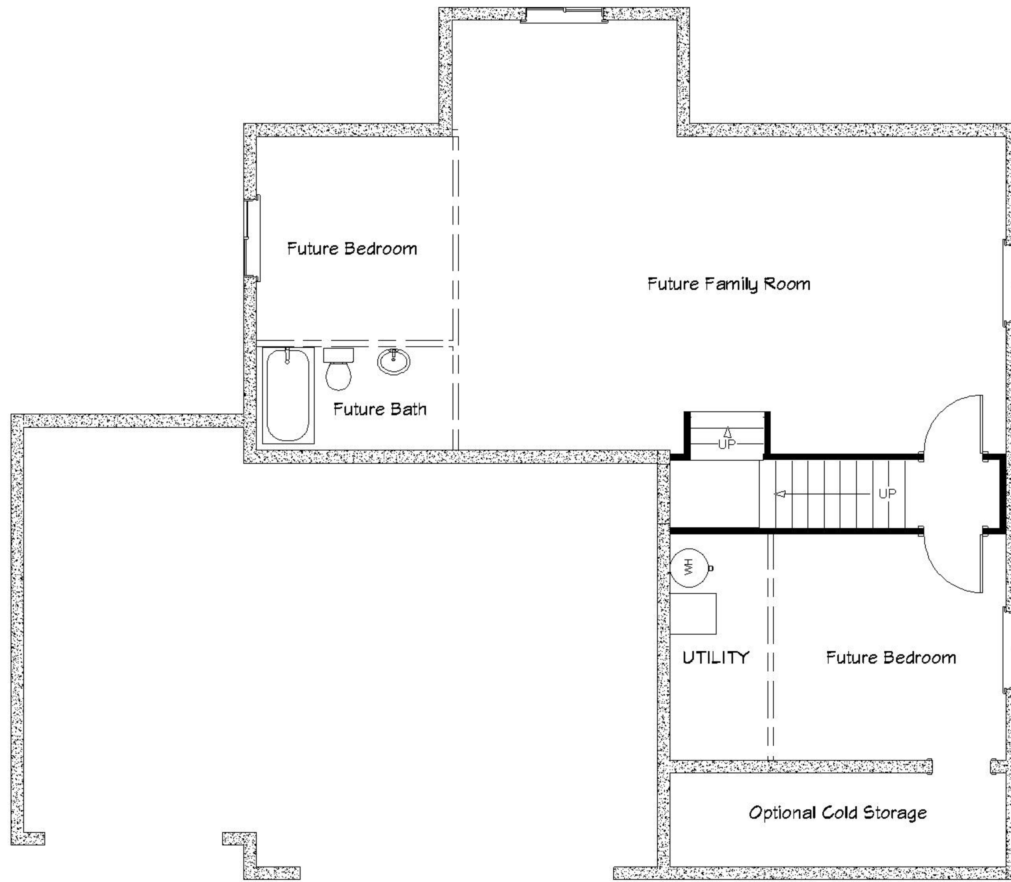
BASEMENT PLAN 1175 Square Feet
