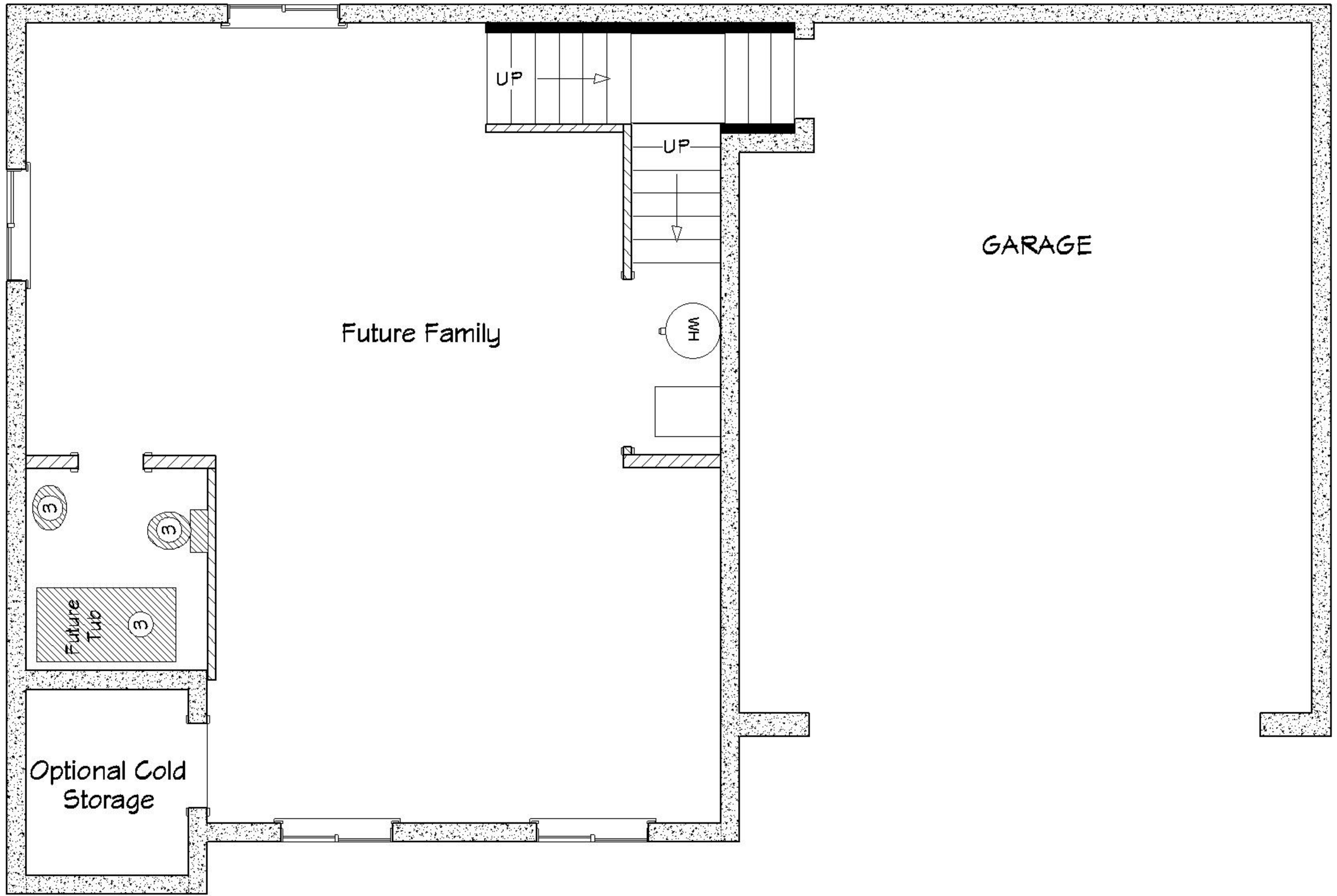
BASEMENT 800 SQUARE FEET
