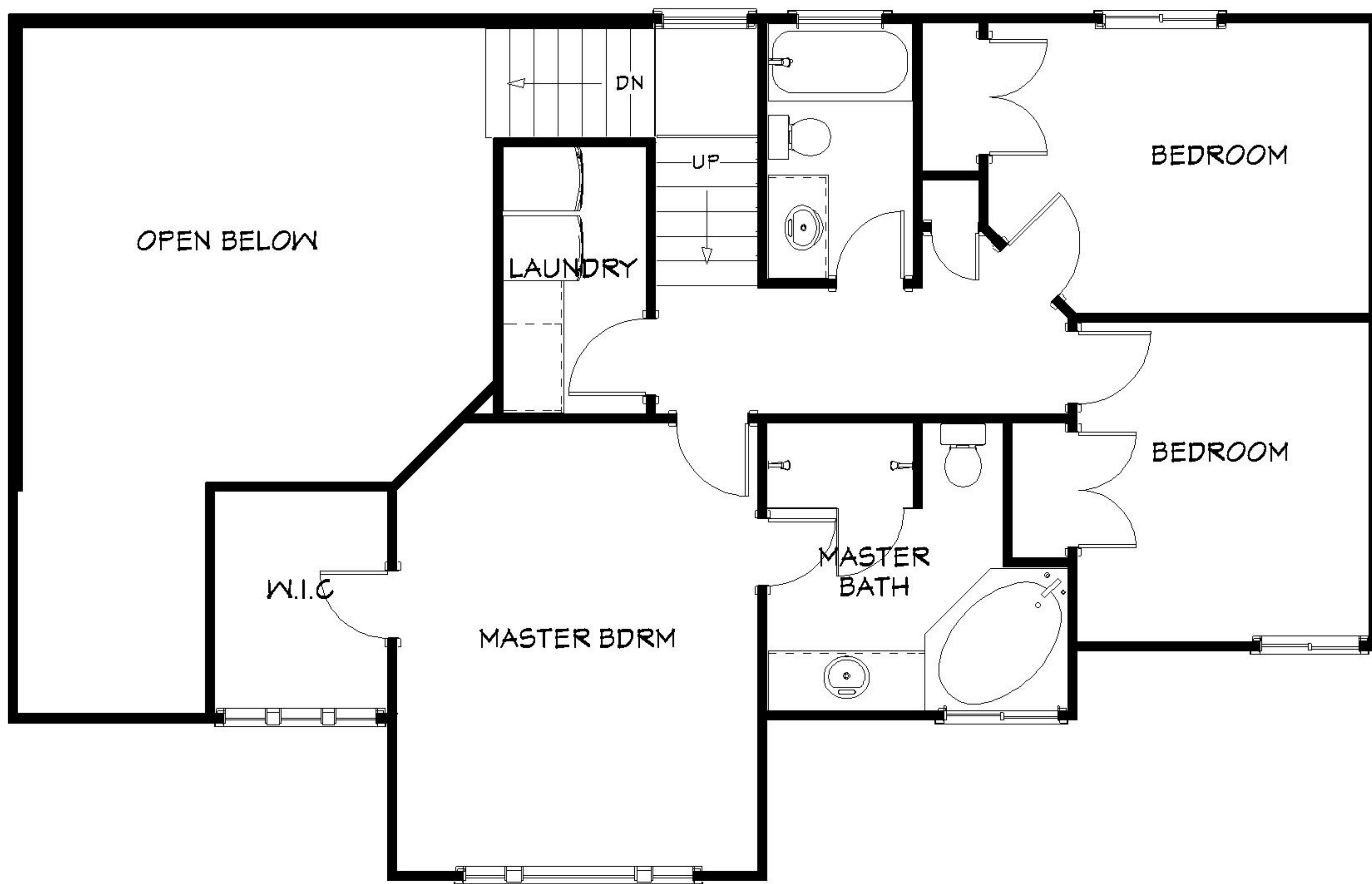
UPPER FLOOR 828 Square Feet
