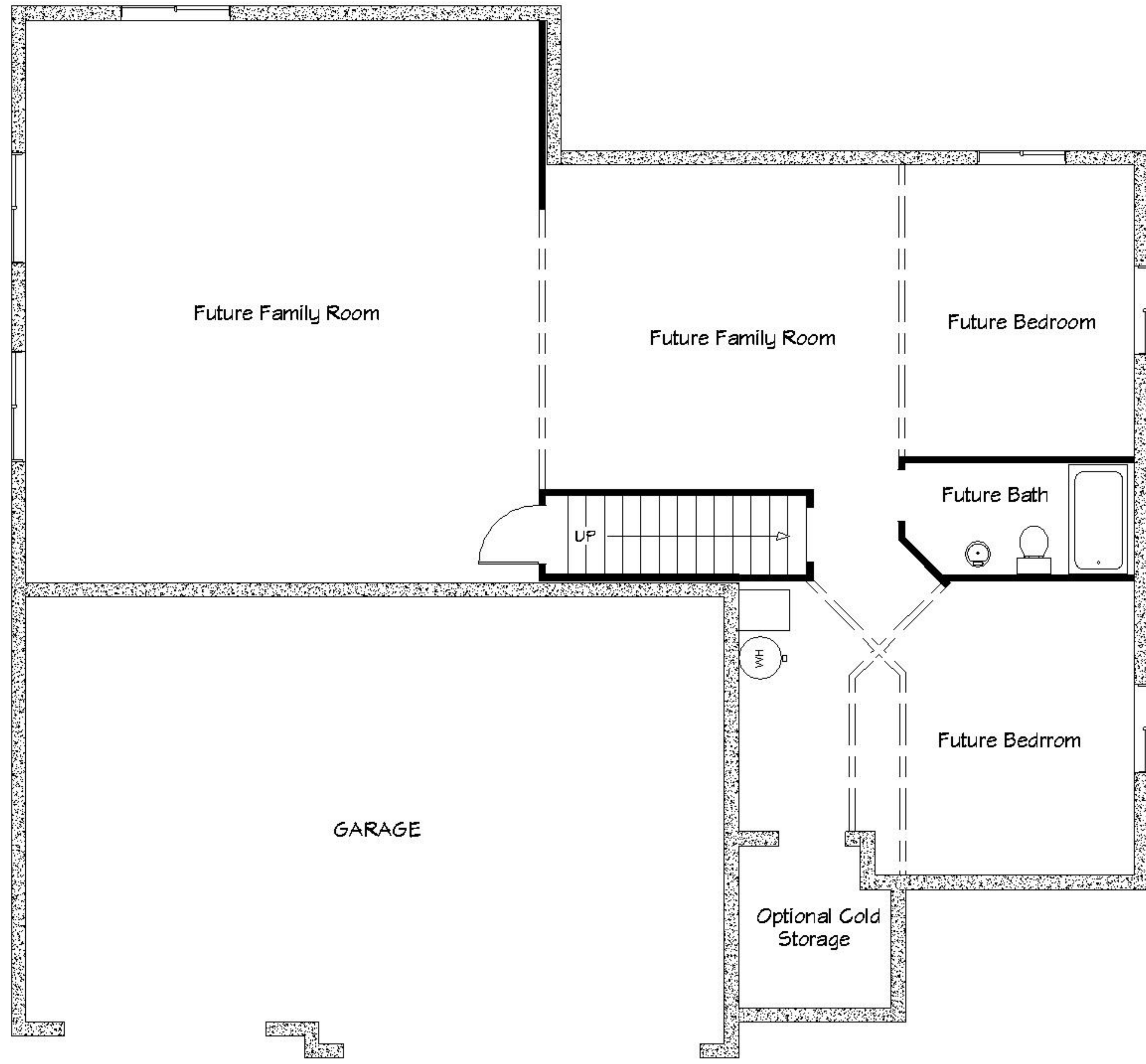
BASEMENT PLAN 1515 square Feet
