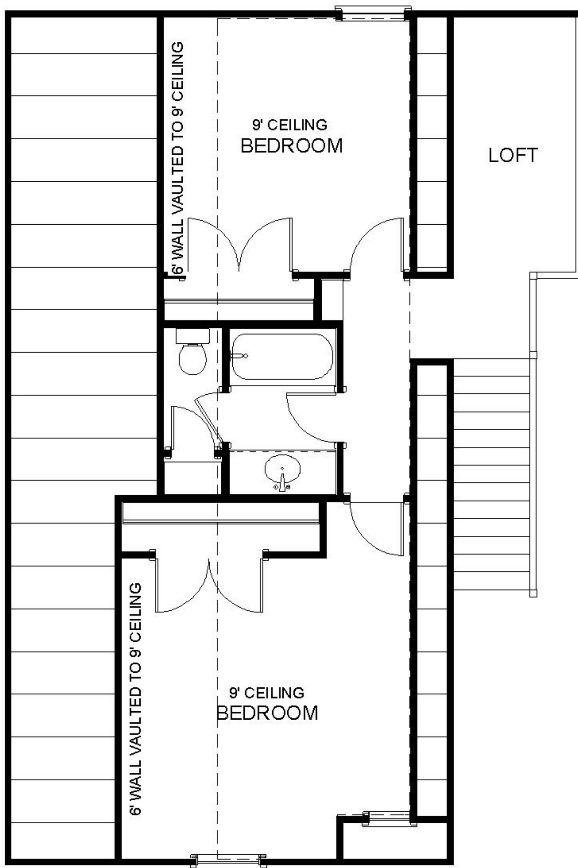
UPPER FLOOR PLAN 603 SQUARE FEET
