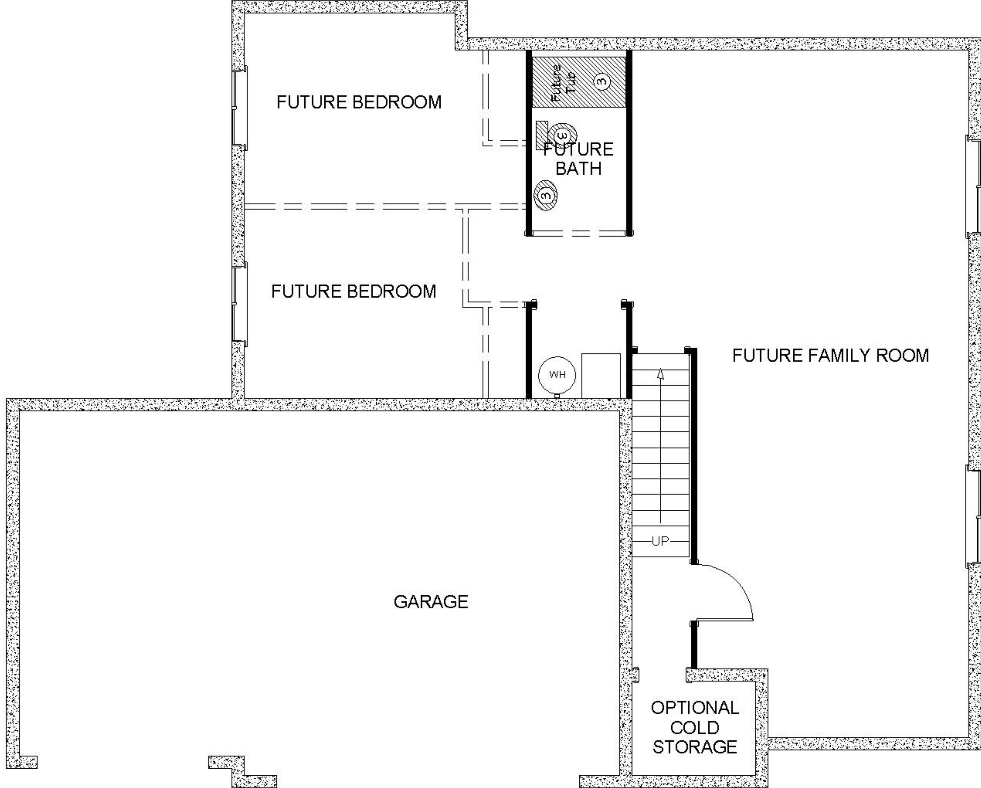
BASEMENT PLAN 1236 SQUARE FEET
