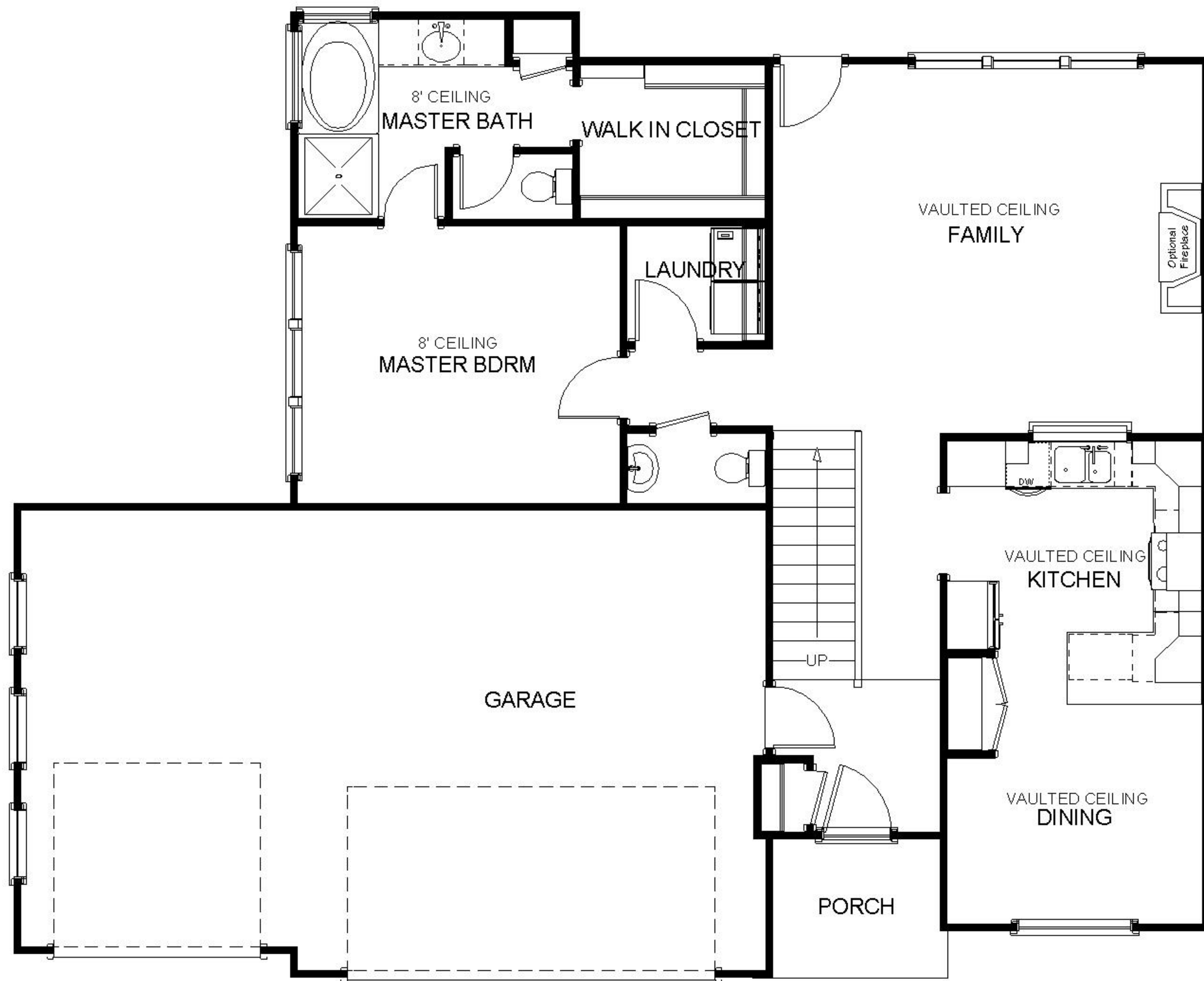
MAIN FLOOR PLAN 1141 SQUARE FEET Width: 52' Depth: 42'
