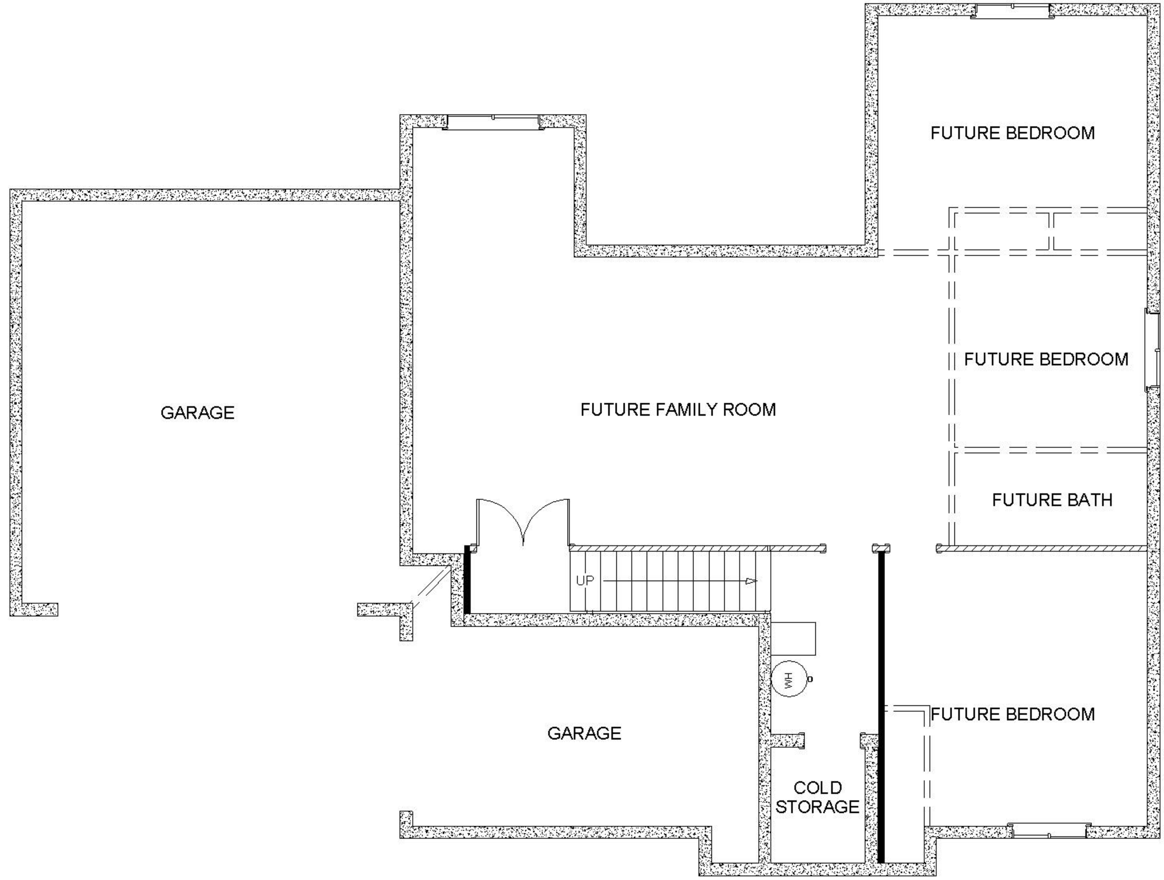
BASEMENT FLOOR PLAN 1366 SQ. FT.
